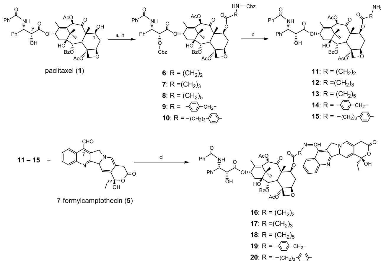
Scheme 1. (a) Benzylchloroformate, pyridine, CH 2 Cl 2 , 83%; (b) N -Cbz-NH-R-COOH, DCC, DMAP, CH 2 Cl 2 , 84–97%; (c) H 2 , 5% Pd-C, MeOH, 81–97%; (d) benzene, MS 4 Å, reflux, 55–85%.
